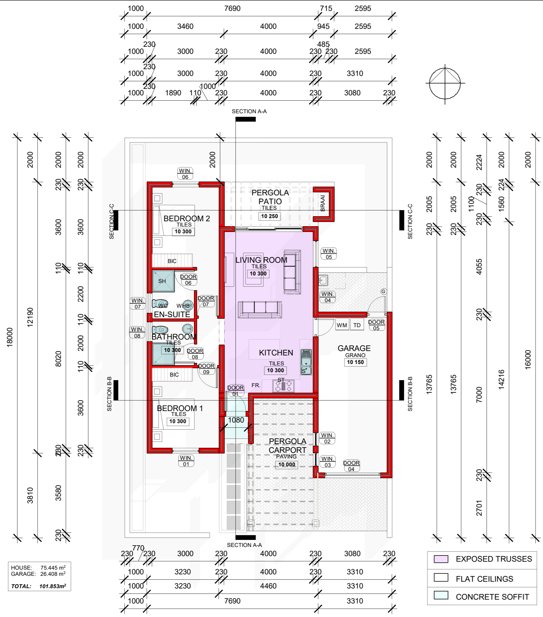
○ GROUND FLOOR 1 : 100
