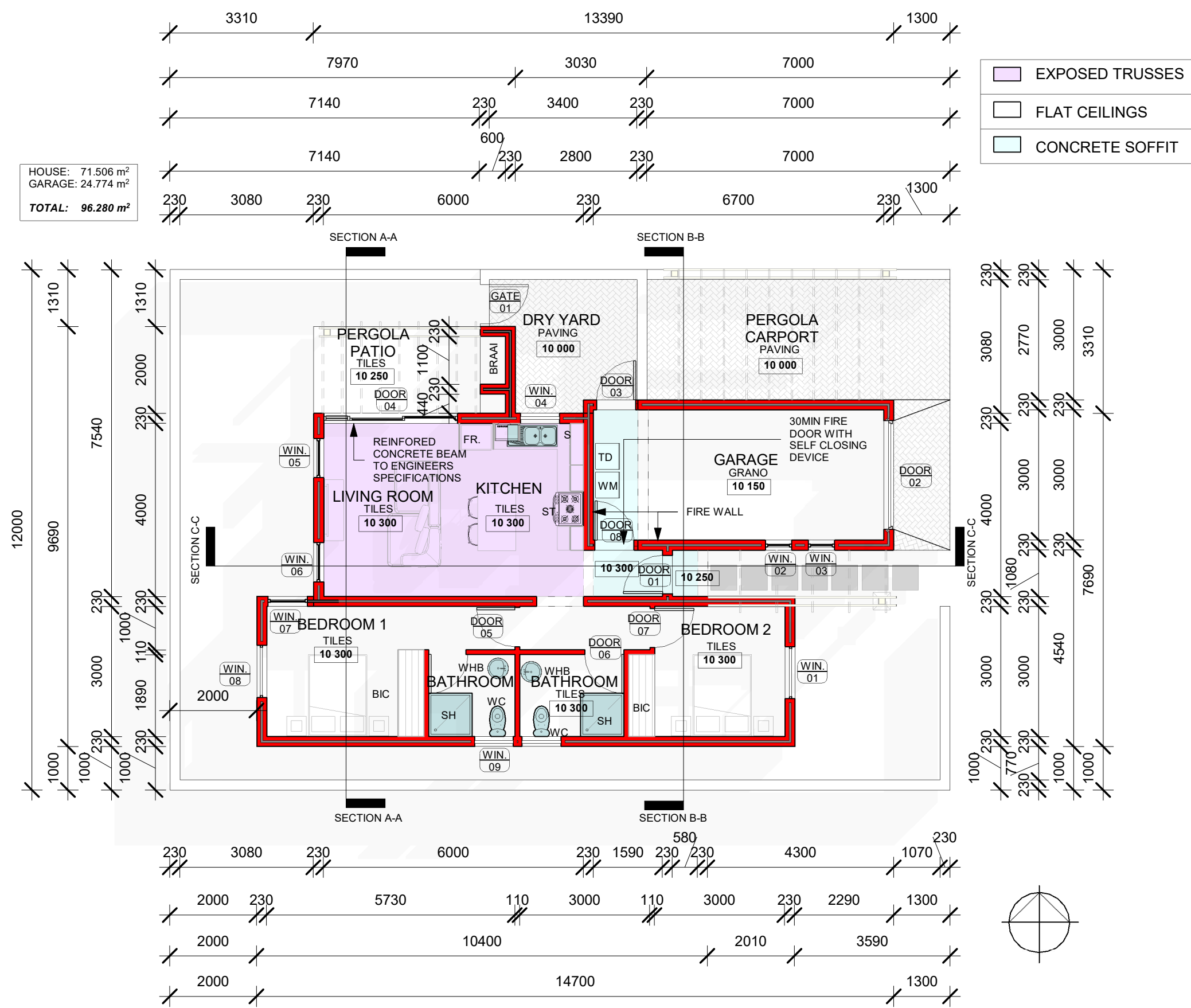
GROUND FLOOR 1 : 100
